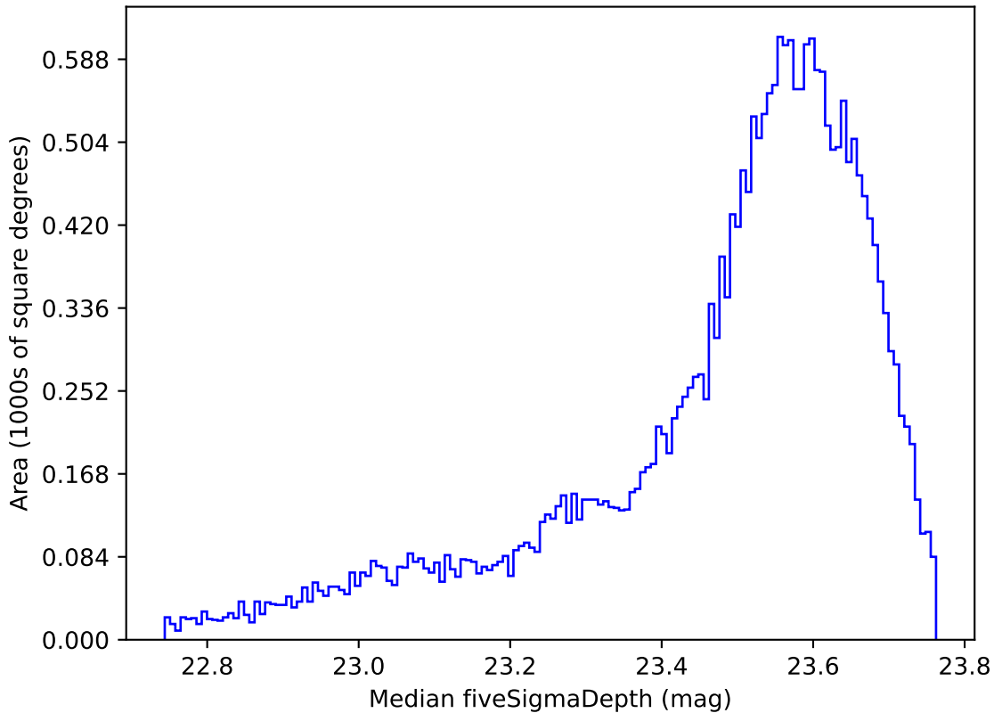
weather_cloudso10v3.4_10yrs All sky i band: Median fiveSigmaDepth
