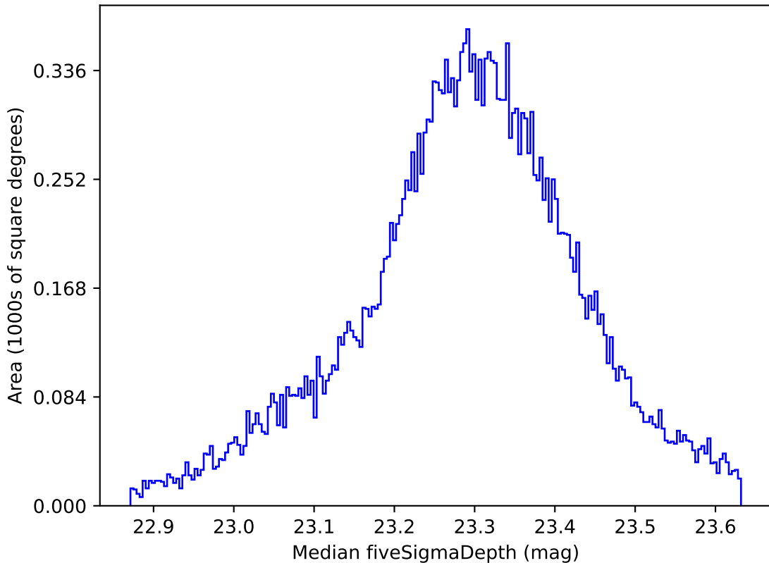
weather_cloudso10v3.4_10yrs All sky all bands: Median fiveSigmaDepth
