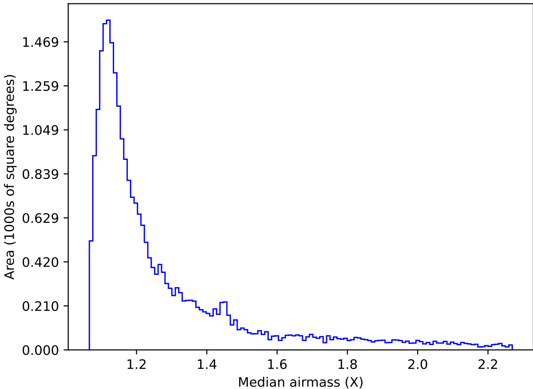
weather_cloudso10v3.4_10yrs Yr 1 z band: Median airmass
