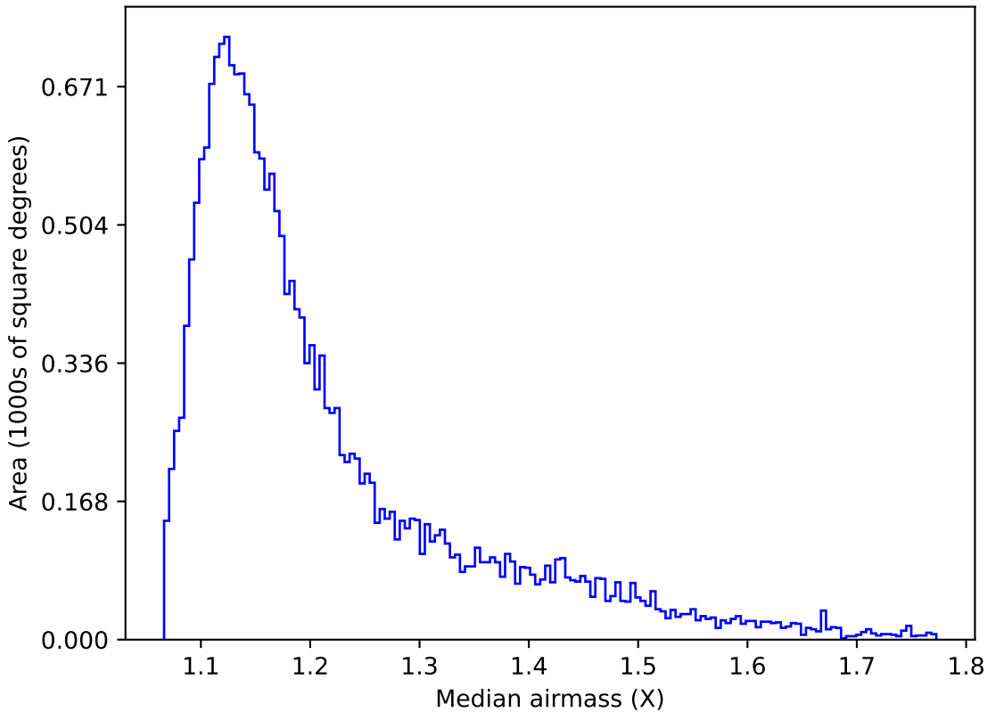
weather_cloudso10v3.4_10yrs Yr 1 y band: Median airmass
