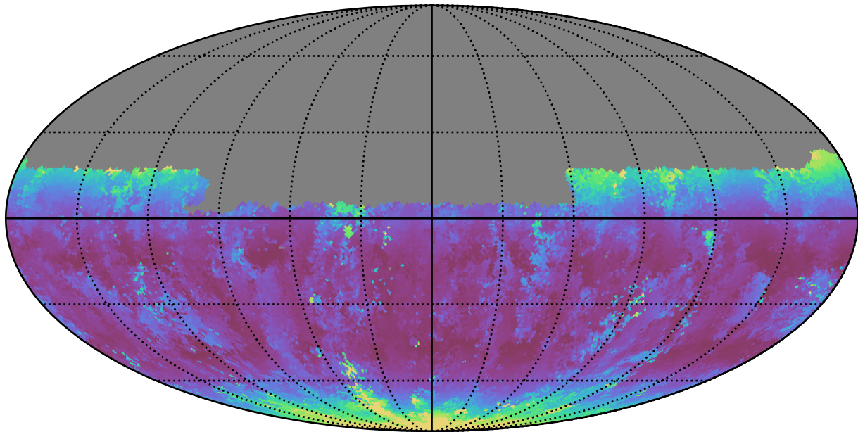
weather_cloudso10v3.4_10yrs Yr 1 u band: Median airmass
