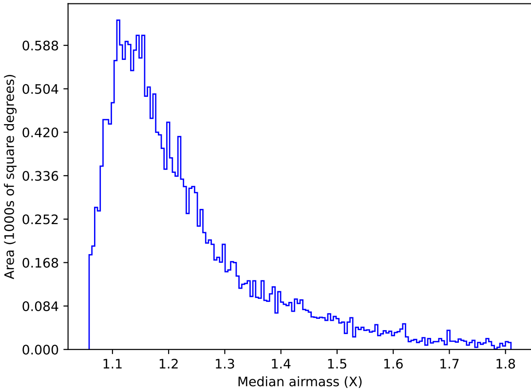
weather_cloudso10v3.4_10yrs Yr 1 u band: Median airmass
