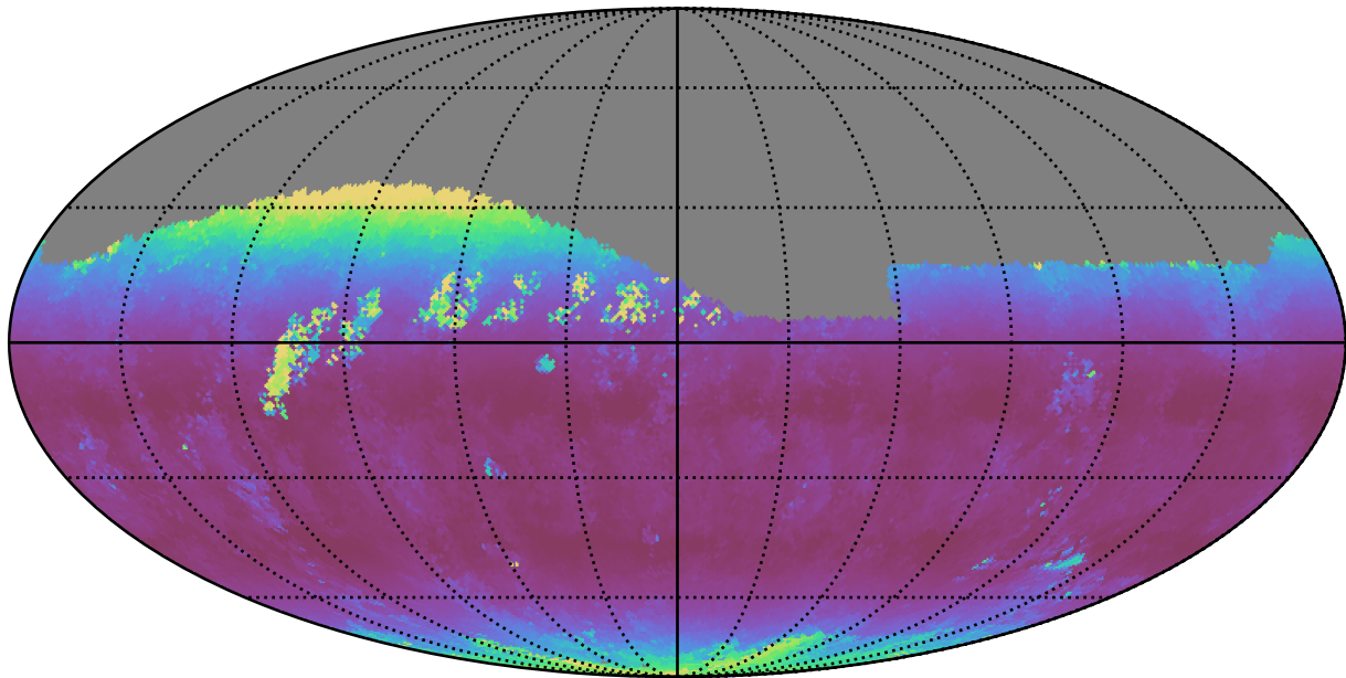
weather_cloudso10v3.4_10yrs Yr 1 r band: Median airmass
