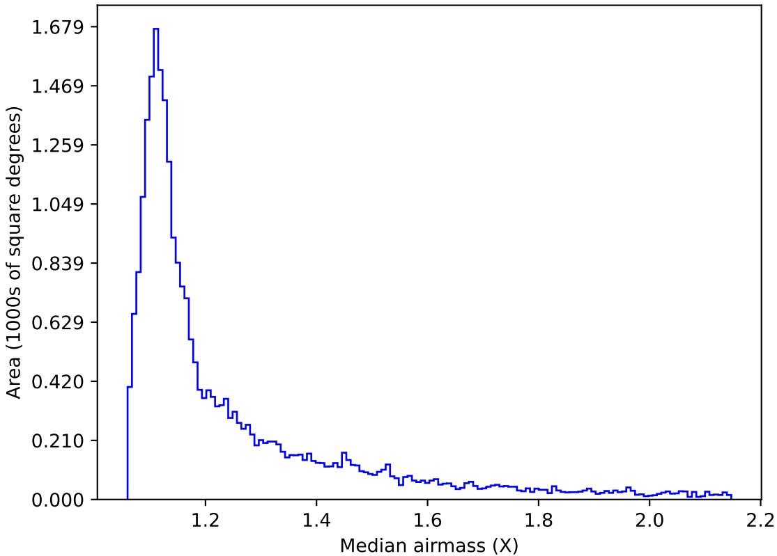
weather_cloudso10v3.4_10yrs Yr 1 r band: Median airmass
