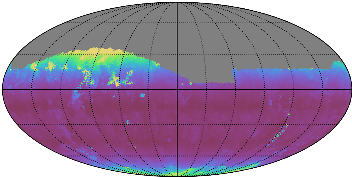
weather_cloudso10v3.4_10yrs Yr 1 i band: Median airmass
