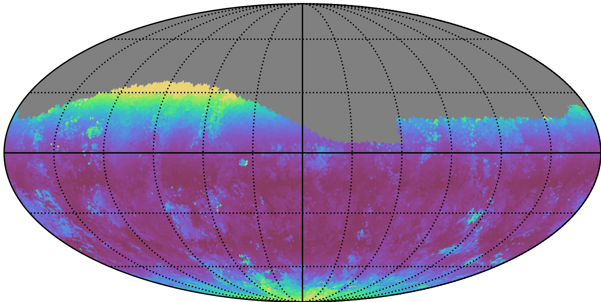
weather_cloudso10v3.4_10yrs Yr 1 g band: Median airmass
