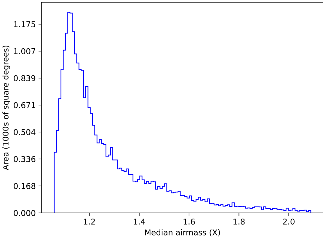
weather_cloudso10v3.4_10yrs Yr 1 g band: Median airmass
