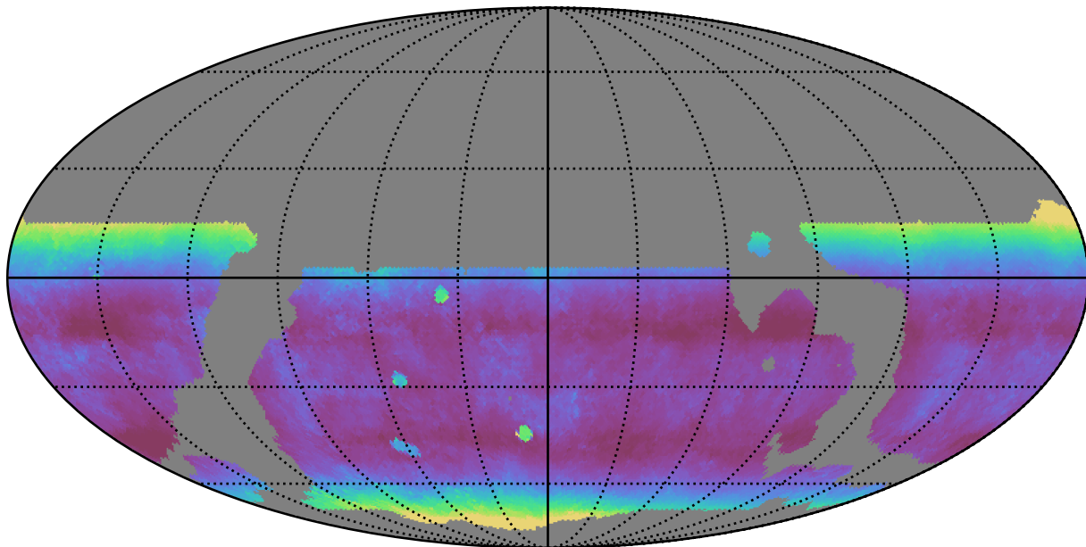
weather_cloudso10v3.4_10yrs WFD z band: Median airmass
