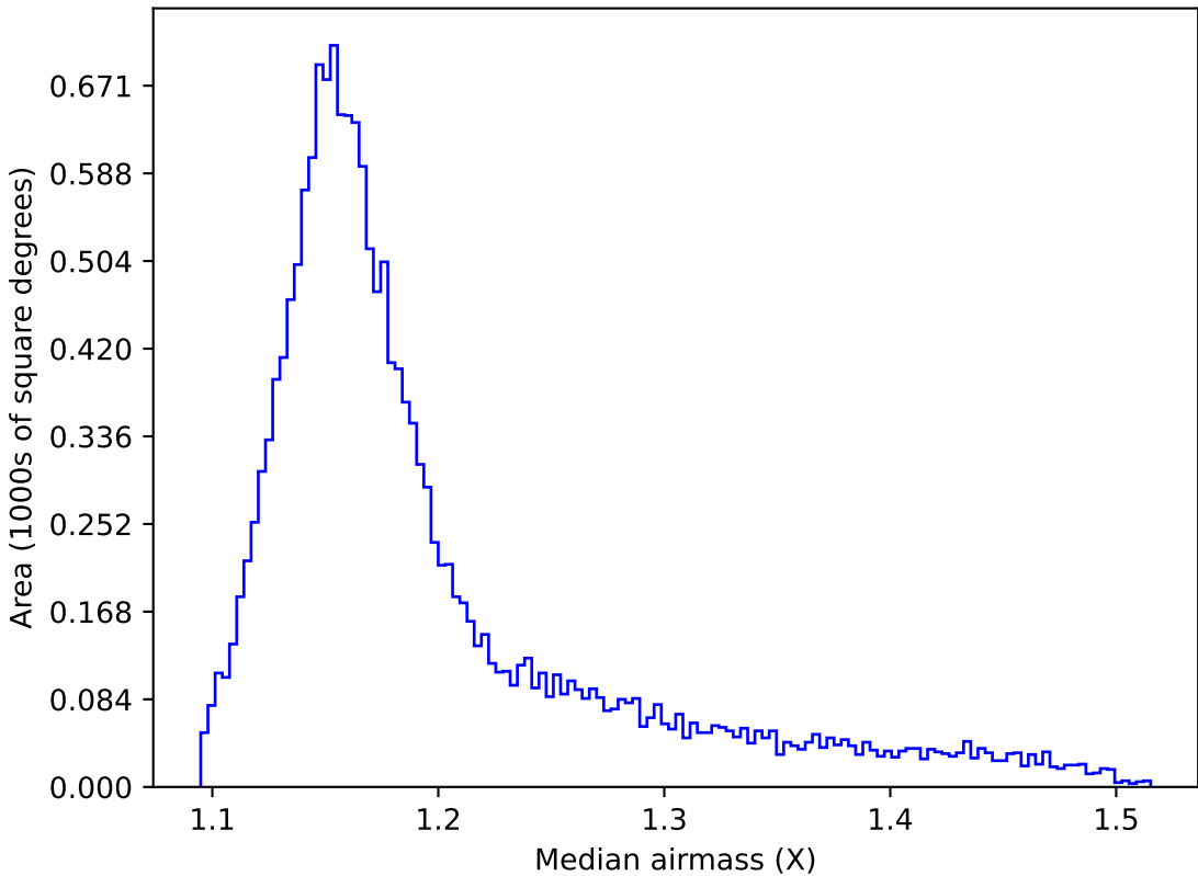
weather_cloudso10v3.4_10yrs WFD z band: Median airmass
