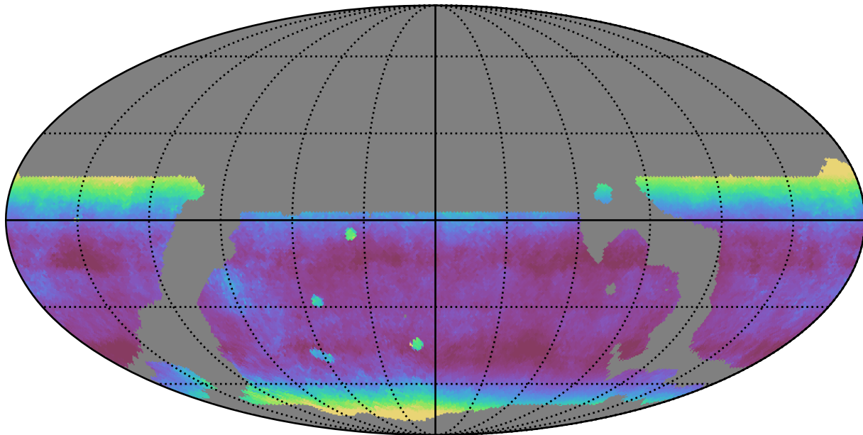
weather_cloudso10v3.4_10yrs WFD y band: Median airmass
