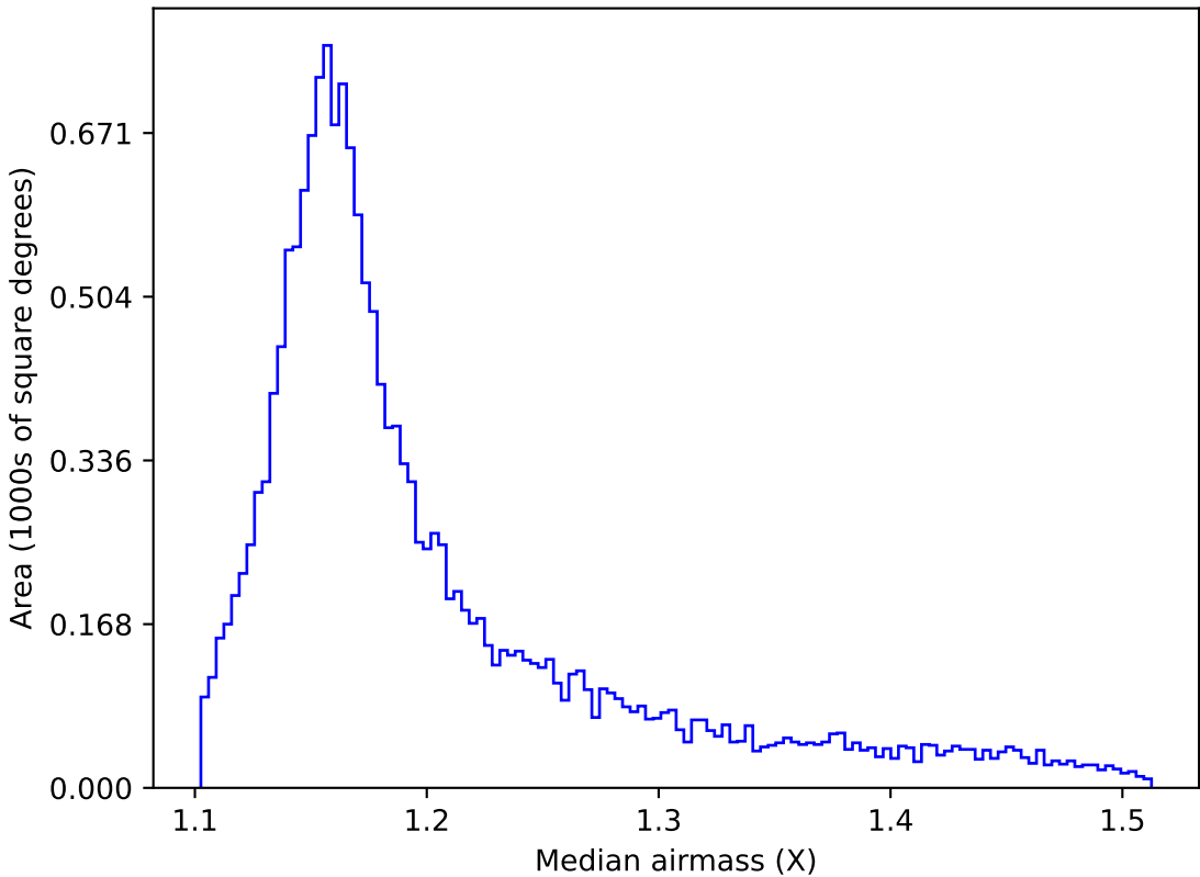
weather_cloudso10v3.4_10yrs WFD y band: Median airmass
