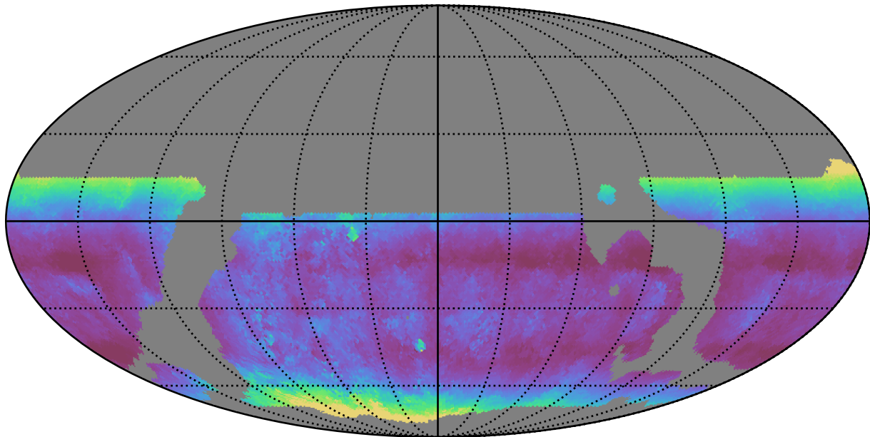
weather_cloudso10v3.4_10yrs WFD u band: Median airmass
