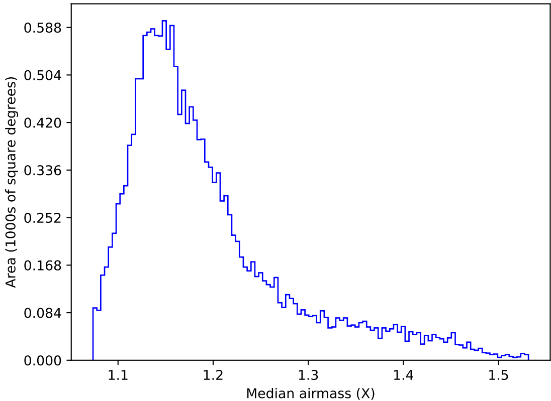
weather_cloudso10v3.4_10yrs WFD u band: Median airmass
