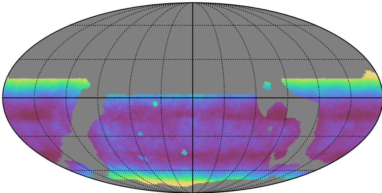
weather_cloudso10v3.4_10yrs WFD r band: Median airmass
