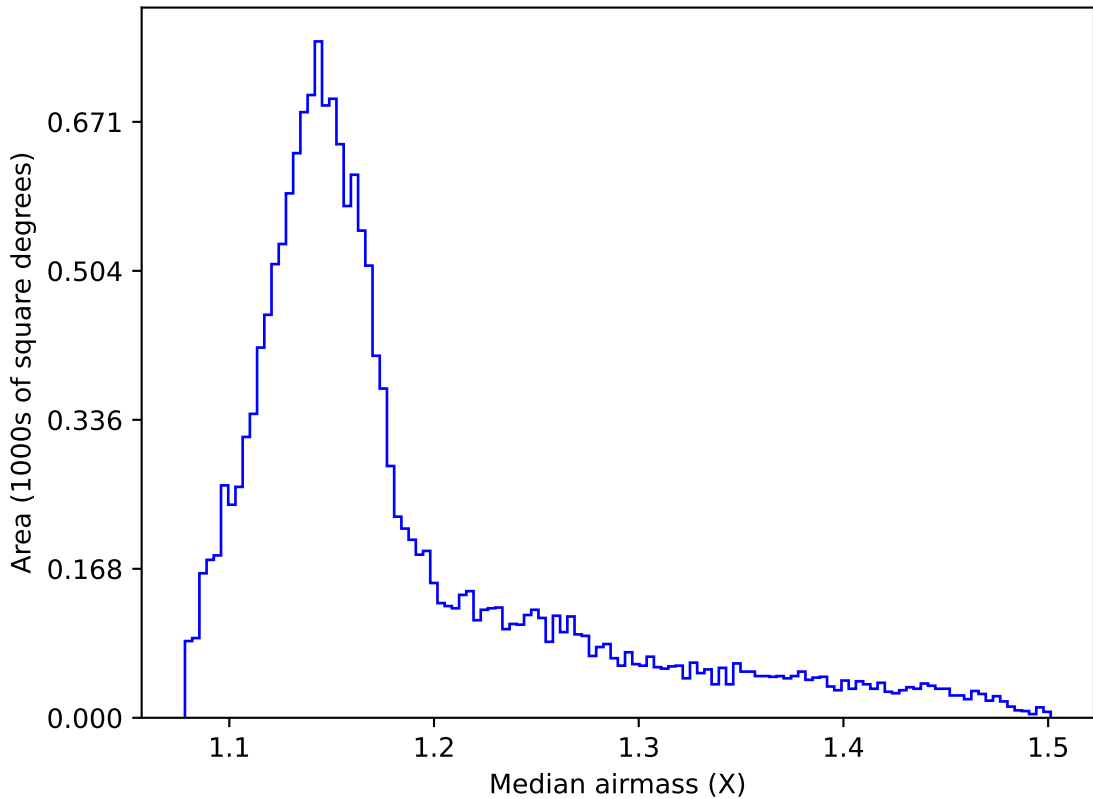
weather_cloudso10v3.4_10yrs WFD r band: Median airmass
