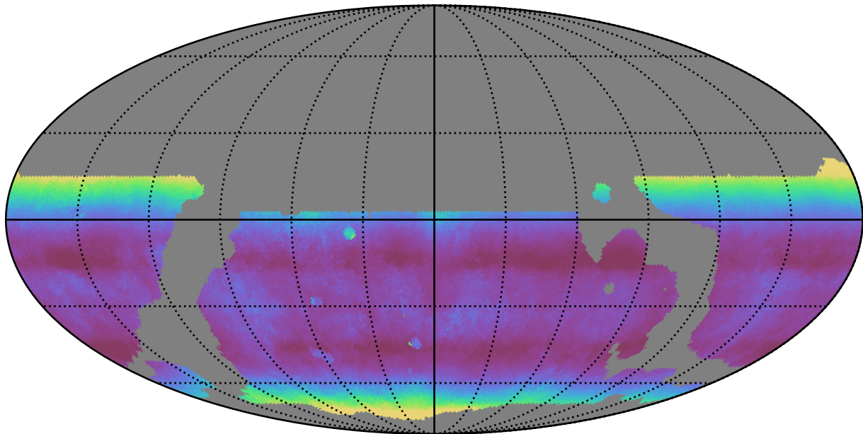
weather_cloudso10v3.4_10yrs WFD i band: Median airmass
