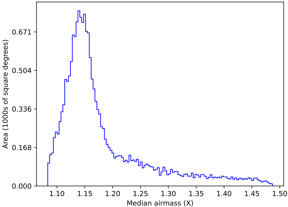
weather_cloudso10v3.4_10yrs WFD i band: Median airmass
