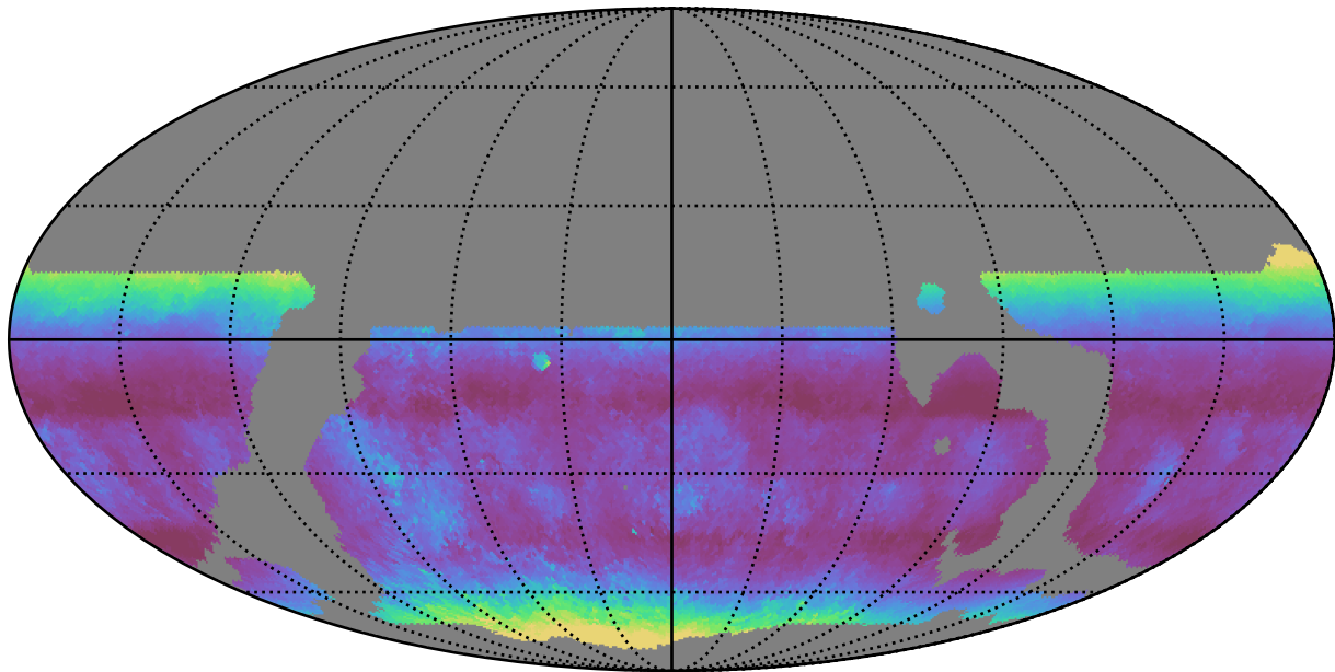
weather_cloudso10v3.4_10yrs WFD g band: Median airmass
