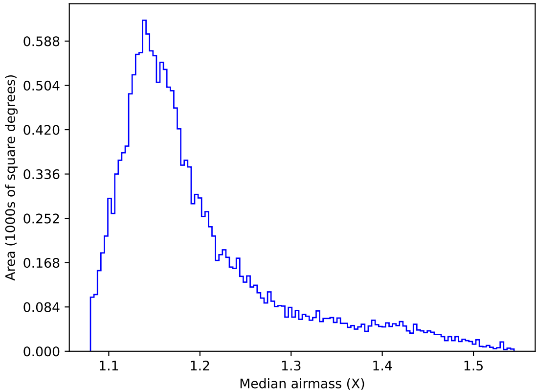
weather_cloudso10v3.4_10yrs WFD g band: Median airmass
