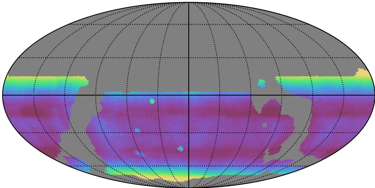
weather_cloudso10v3.4_10yrs WFD all bands: Median airmass
