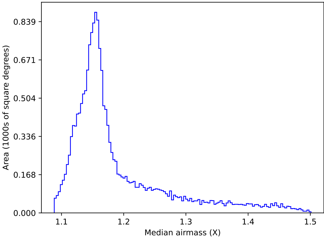
weather_cloudso10v3.4_10yrs WFD all bands: Median airmass
