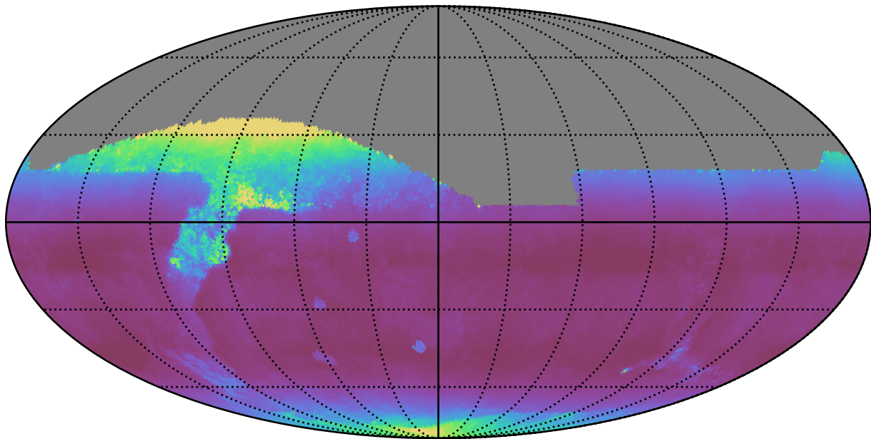
weather_cloudso10v3.4_10yrs All sky z band: Median airmass
