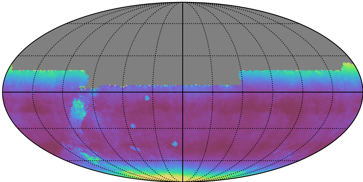
weather_cloudso10v3.4_10yrs All sky y band: Median airmass
