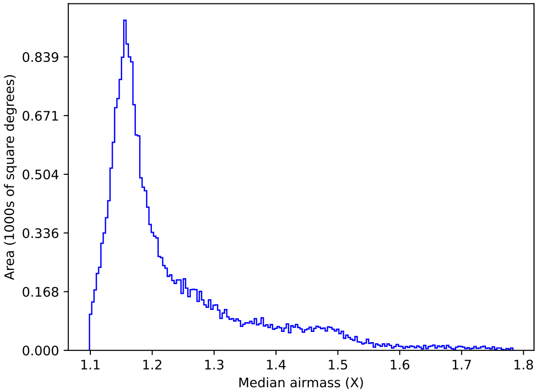
weather_cloudso10v3.4_10yrs All sky y band: Median airmass
