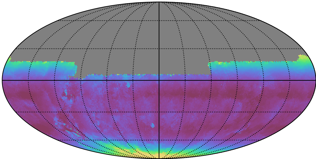
weather_cloudso10v3.4_10yrs All sky u band: Median airmass
