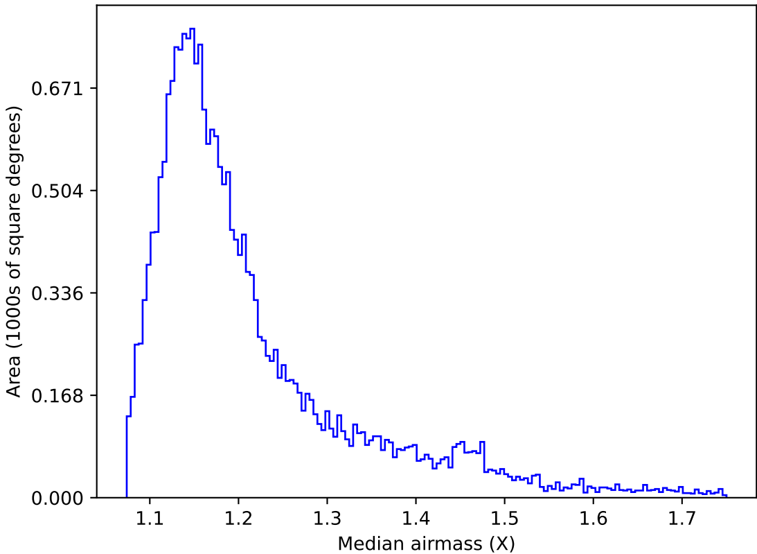
weather_cloudso10v3.4_10yrs All sky u band: Median airmass
