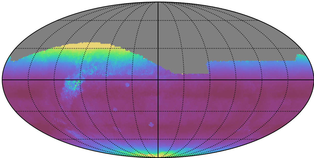
weather_cloudso10v3.4_10yrs All sky r band: Median airmass
