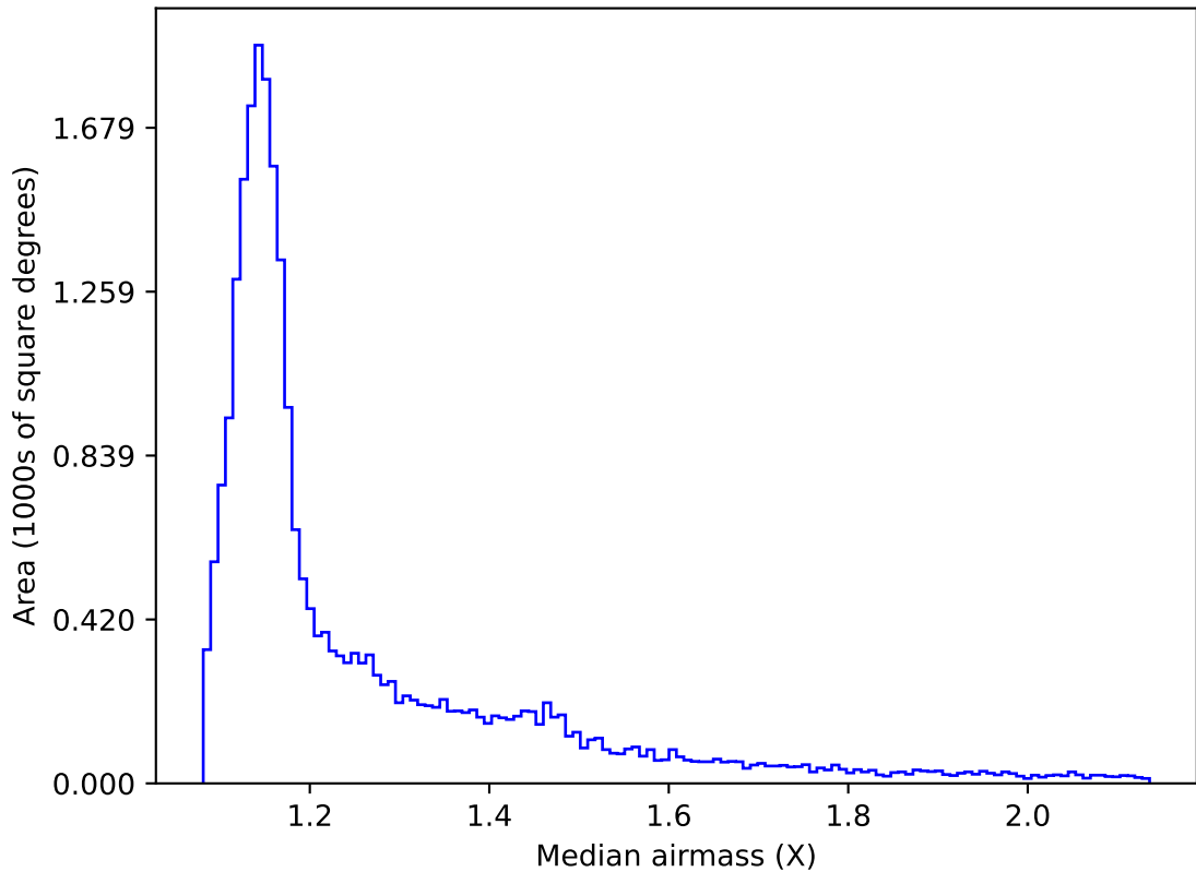
weather_cloudso10v3.4_10yrs All sky r band: Median airmass
