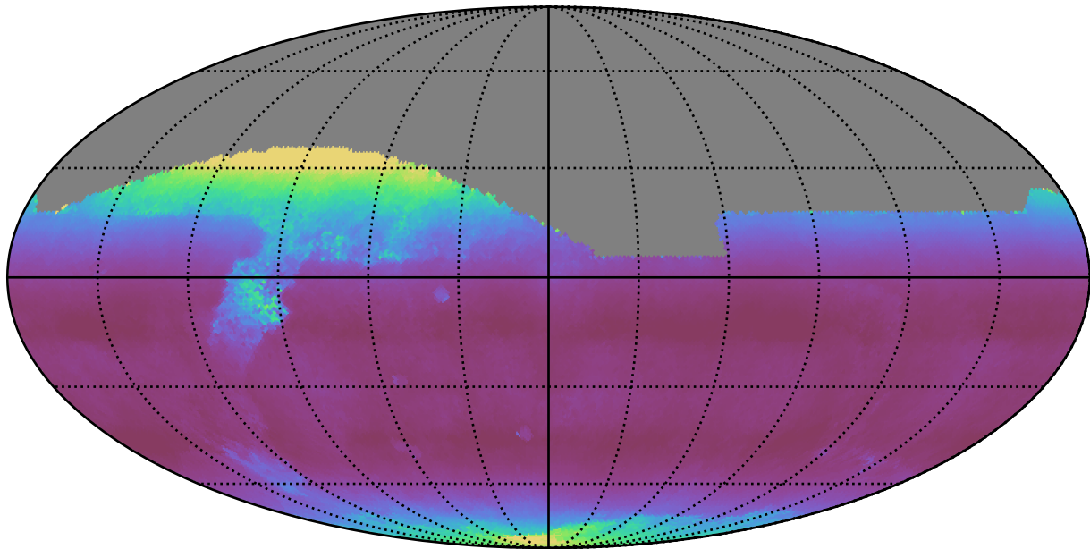
weather_cloudso10v3.4_10yrs All sky i band: Median airmass
