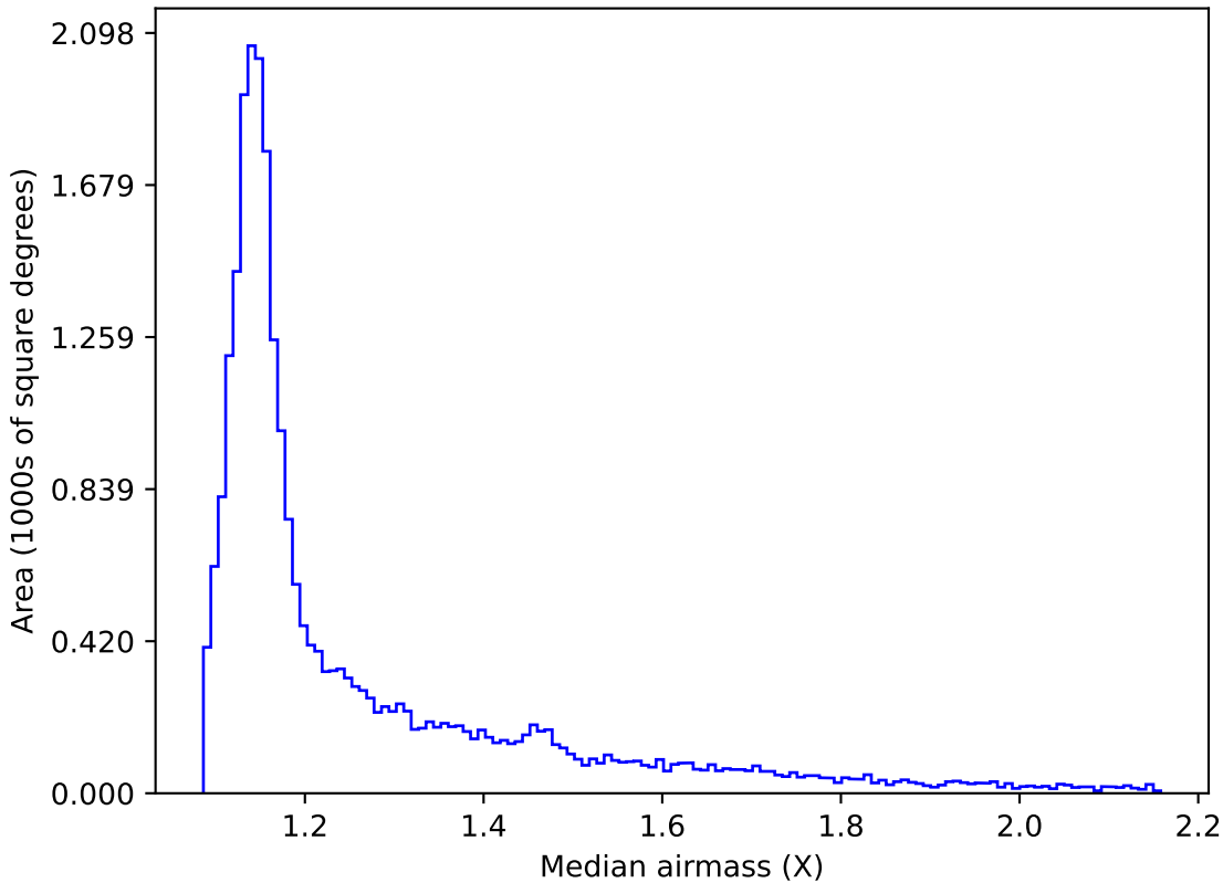
weather_cloudso10v3.4_10yrs All sky i band: Median airmass
