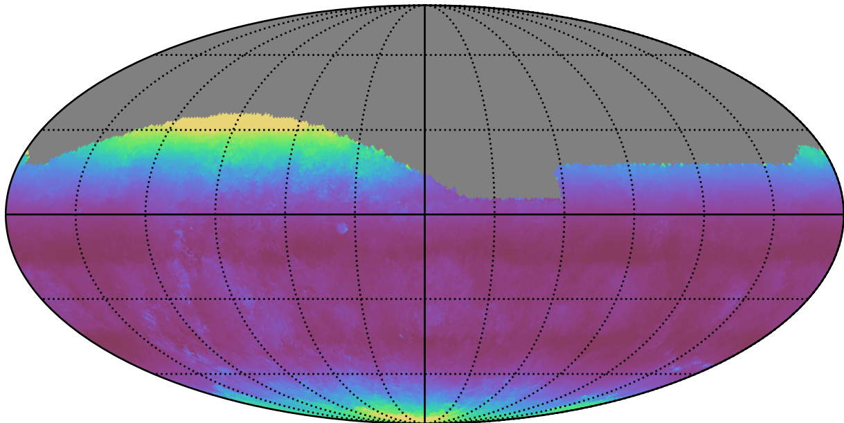
weather_cloudso10v3.4_10yrs All sky g band: Median airmass
