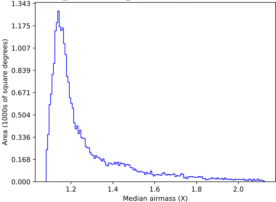
weather_cloudso10v3.4_10yrs All sky g band: Median airmass
