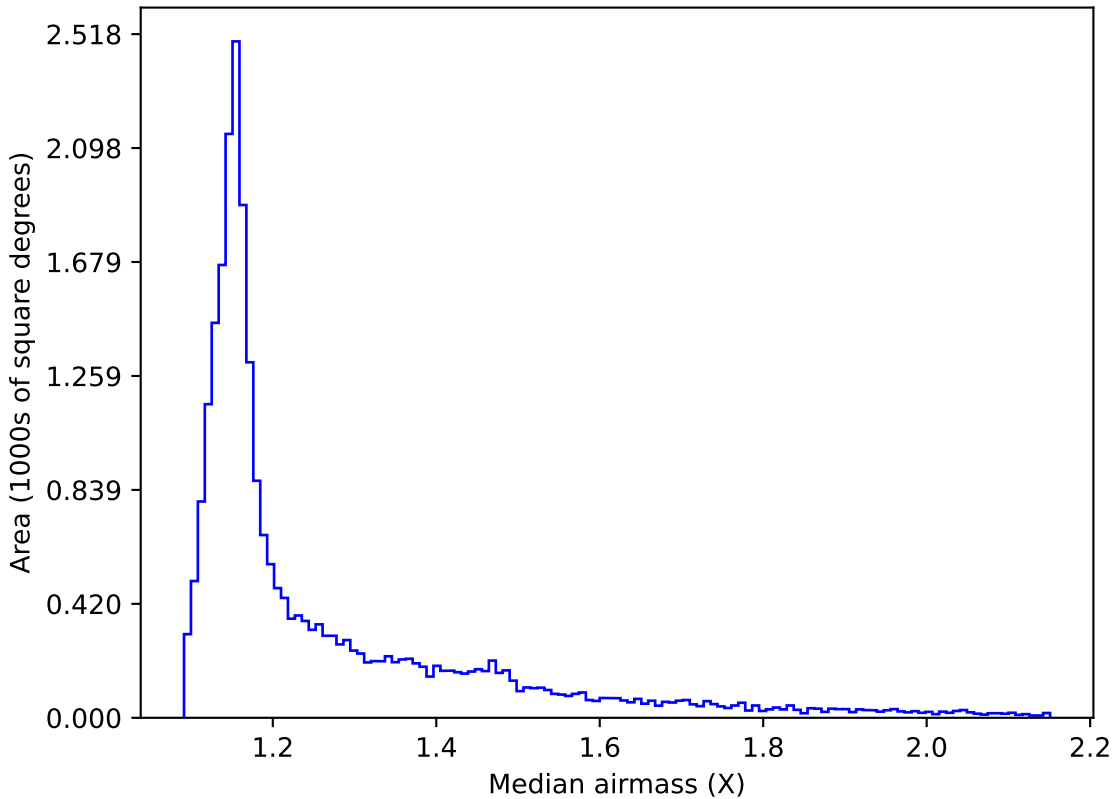
weather_cloudso10v3.4_10yrs All sky all bands: Median airmass
