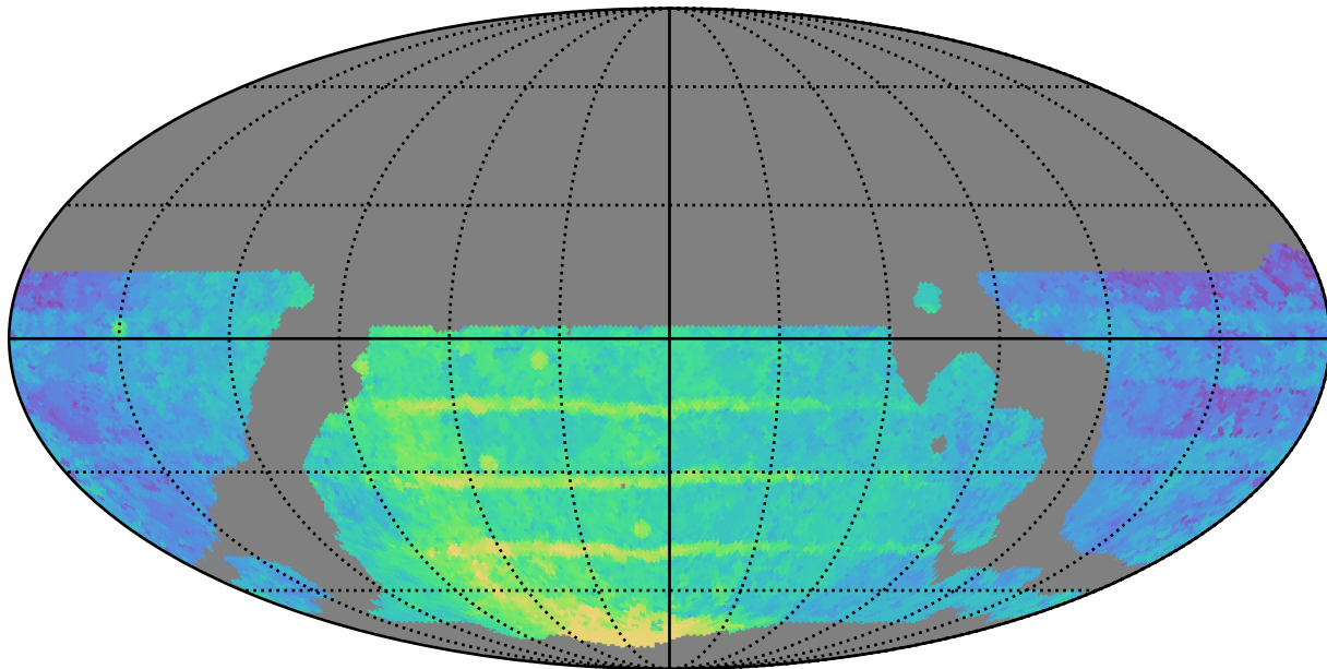
weather_cloudso10v3.4_10yrs WFD z band: Median Season Length
