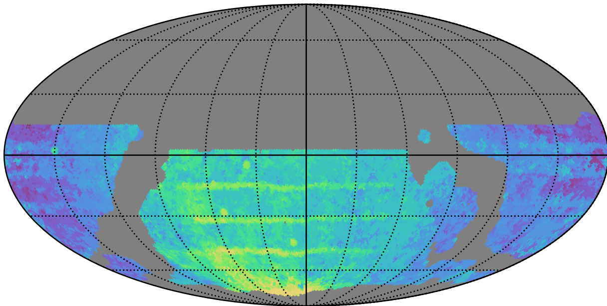
weather_cloudso10v3.4_10yrs WFD y band: Median Season Length
