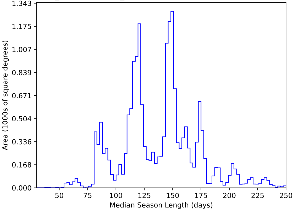
weather_cloudso10v3.4_10yrs WFD y band: Median Season Length
