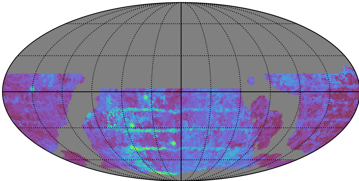
weather_cloudso10v3.4_10yrs WFD u band: Median Season Length
