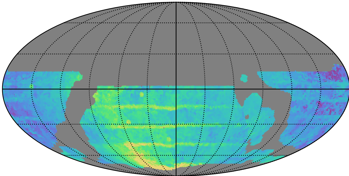
weather_cloudso10v3.4_10yrs WFD r band: Median Season Length
