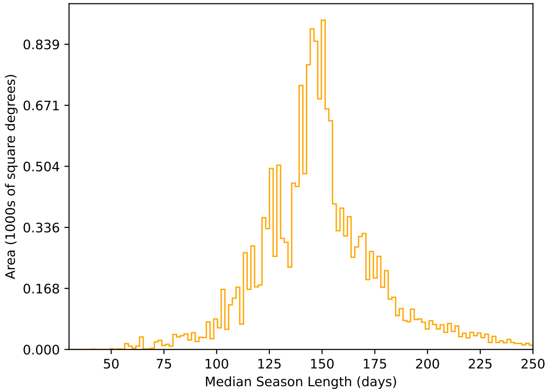
weather_cloudso10v3.4_10yrs WFD r band: Median Season Length
