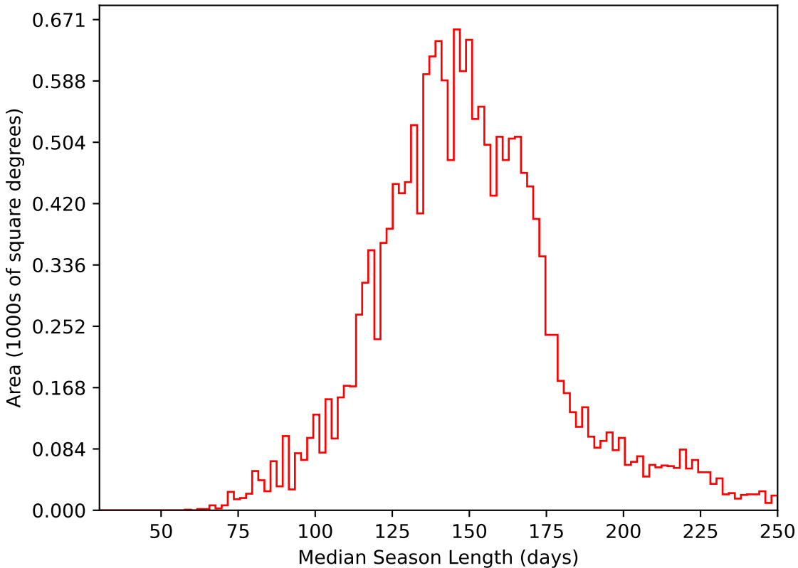
weather_cloudso10v3.4_10yrs WFD i band: Median Season Length
