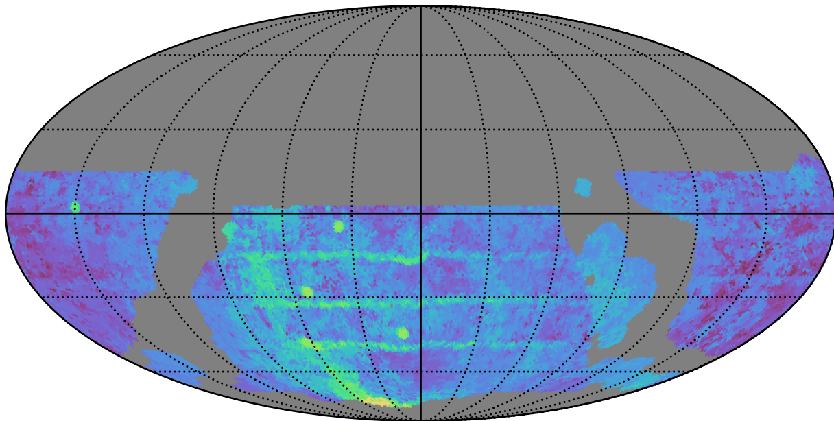
weather_cloudso10v3.4_10yrs WFD g band: Median Season Length
