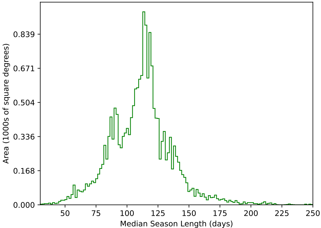
weather_cloudso10v3.4_10yrs WFD g band: Median Season Length
