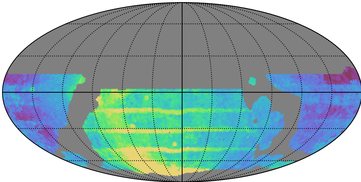
weather_cloudso10v3.4_10yrs WFD all bands: Median Season Length
