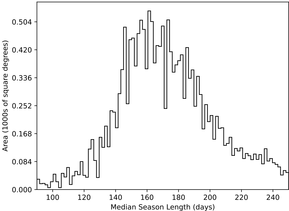
weather_cloudso10v3.4_10yrs WFD all bands: Median Season Length
