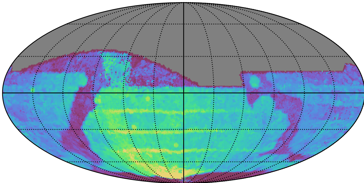
weather_cloudso10v3.4_10yrs All sky z band: Median Season Length
