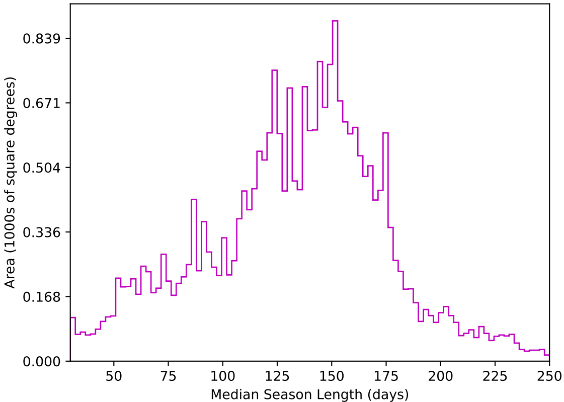
weather_cloudso10v3.4_10yrs All sky z band: Median Season Length
